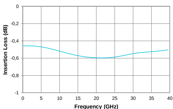
Insertion Loss
